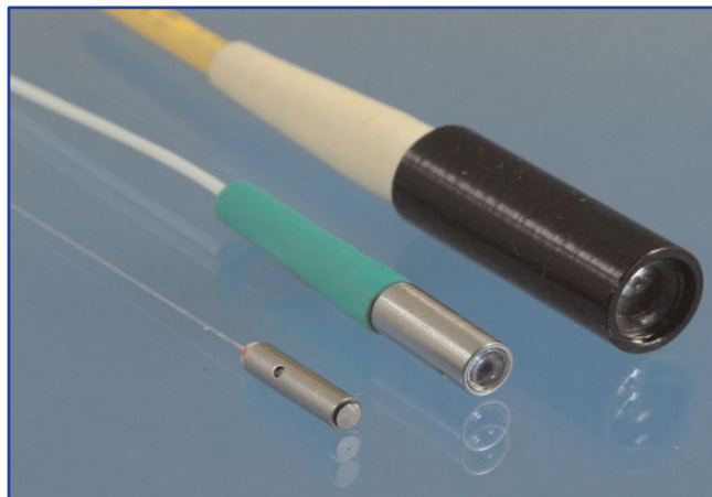
2.5 mm, 4 mm, and 8 mm OD Collimators / Focusers
