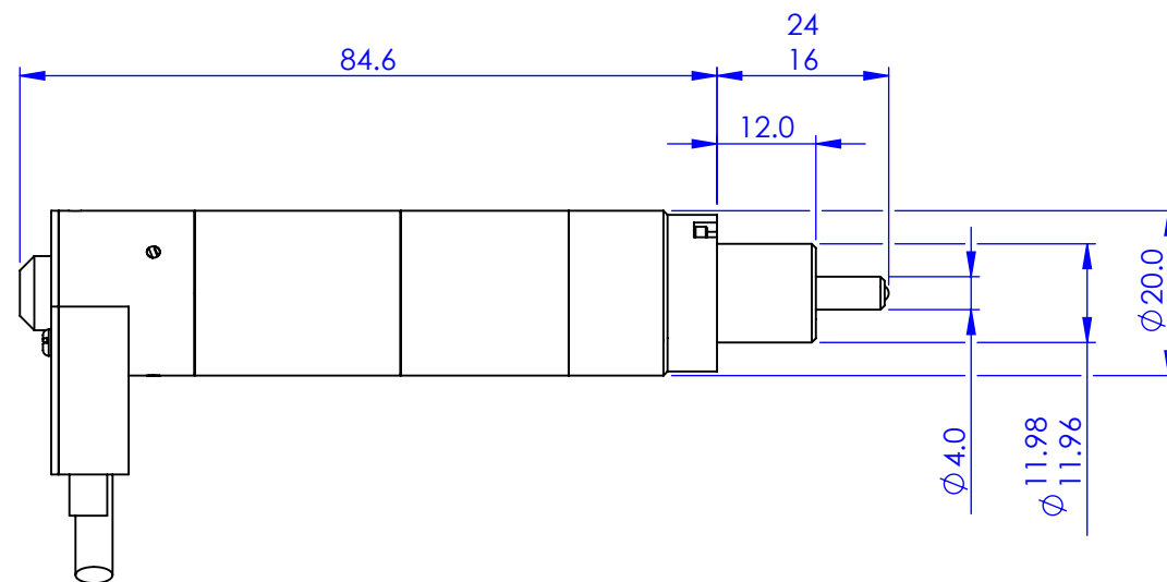
GENERAL VIEW SCALE 1:1
